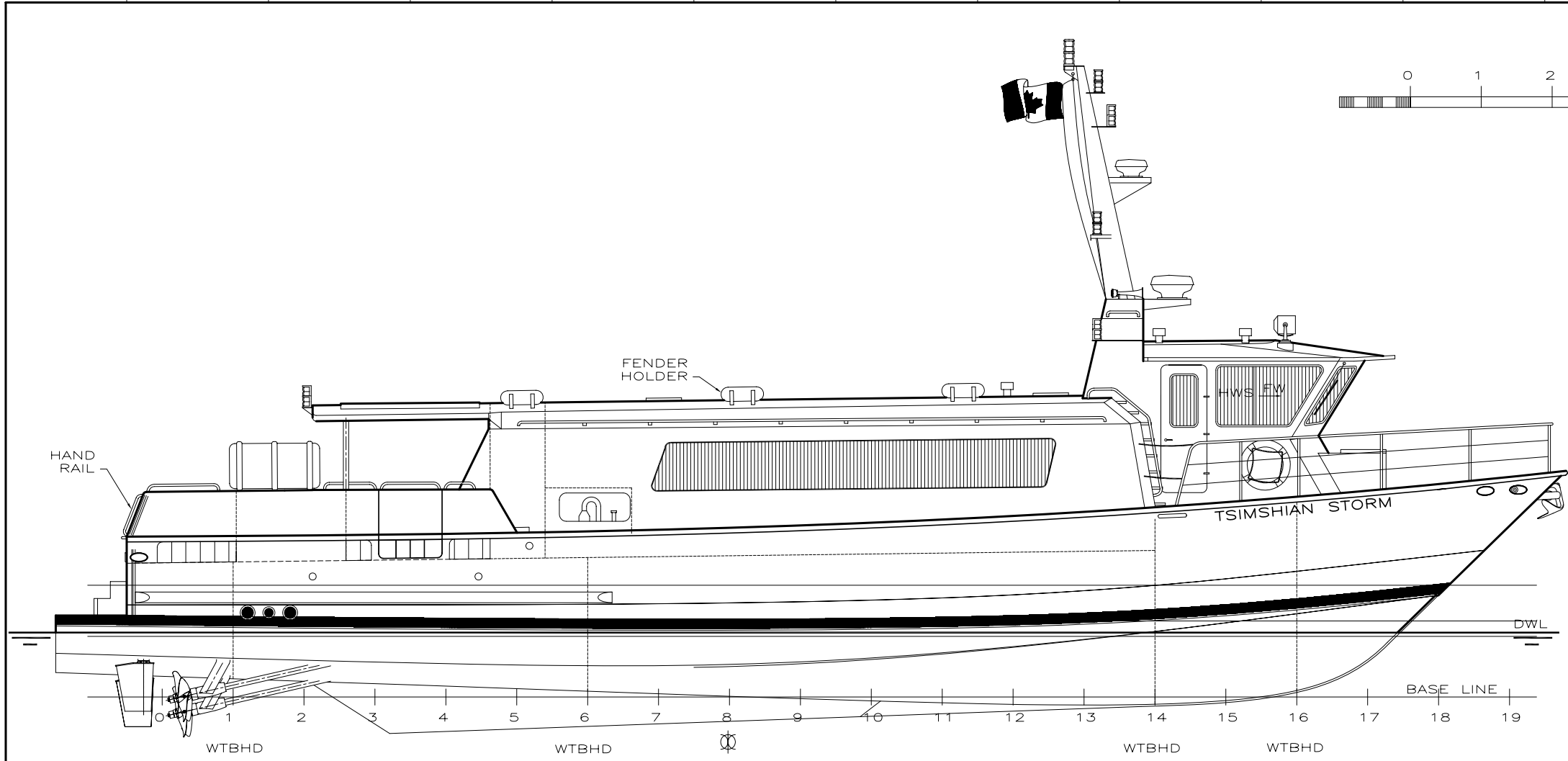
OUTBOARD PROFILE
